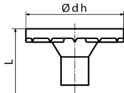
Flat washer head with or without under head ribs with or without neck
