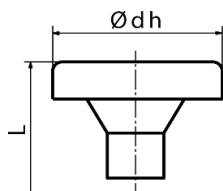
PAN head with or without neck
