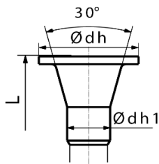
Jet head
