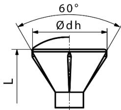
Trimkopf with or without lens, with or without milling pockets/milling ribs
