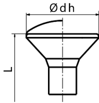
Countersunk head with or without lense, with or without milling pockets/milling ribs
