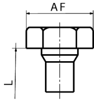
Hexagon head with or without neck
