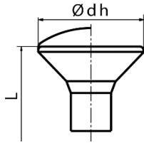
Countersunk head with or without lense, with or without milling pockets/milling ribs
